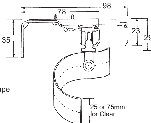
Single Centre Support Bracket No 5255
