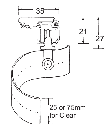
Small Ceiling Bracket No 5253
