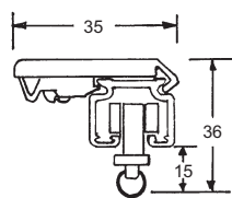
Small Ceiling Bracket No 5253
