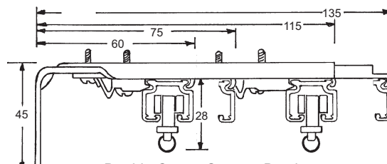
Double Centre Support Bracket No 5255S
