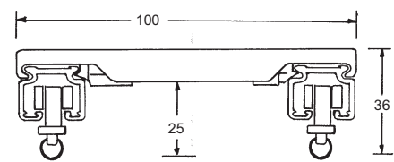
Double Ceiling Bracket No 5258
