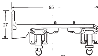
95mm Fixed Projection Double Bracket No 5254
