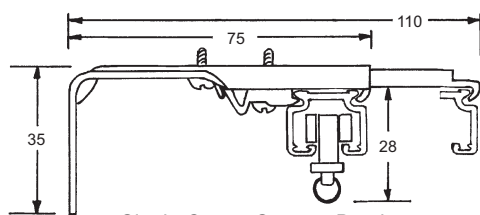
Single Centre Support Bracket No 5255
