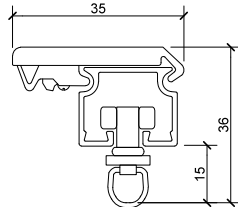
SERIES 52 Ceiling Bracket No 5253
