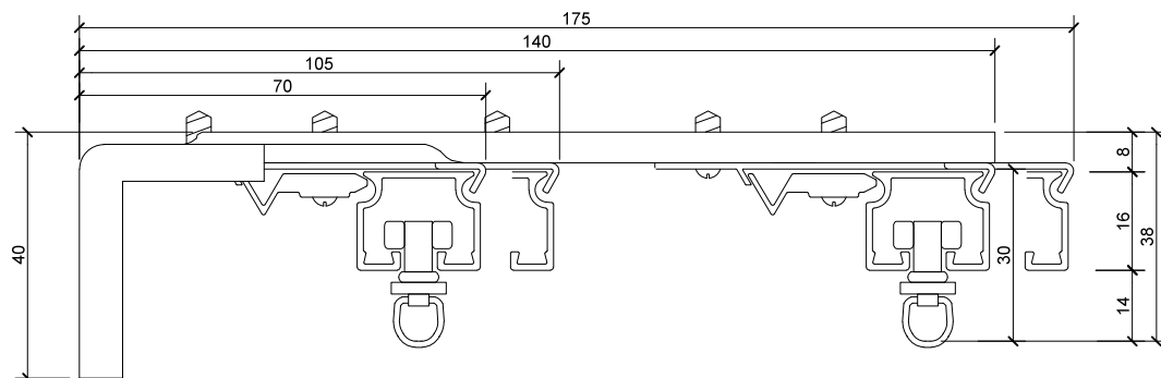
SERIES 52 Double Centre Support Bracket No 52455L
