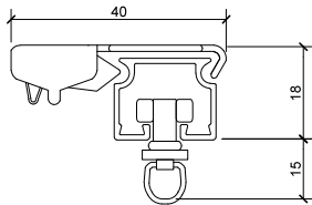
SERIES 52 Ceiling Bracket No 5153L
