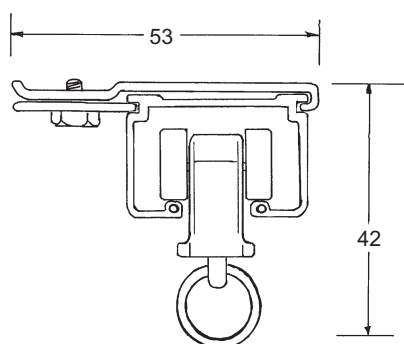
Ceiling Fix Bracket No 5353
