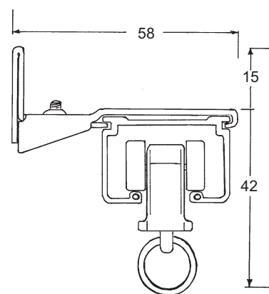
Face Fix Bracket No 5351
