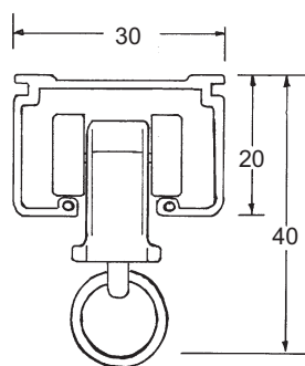
Light Stage Track Section
